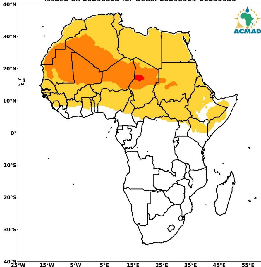
VIGILANCE MAP FOR MENINGITIS OUTBREAKS IN AFRICA issued on 20230323 for week: 20230324-20230330
