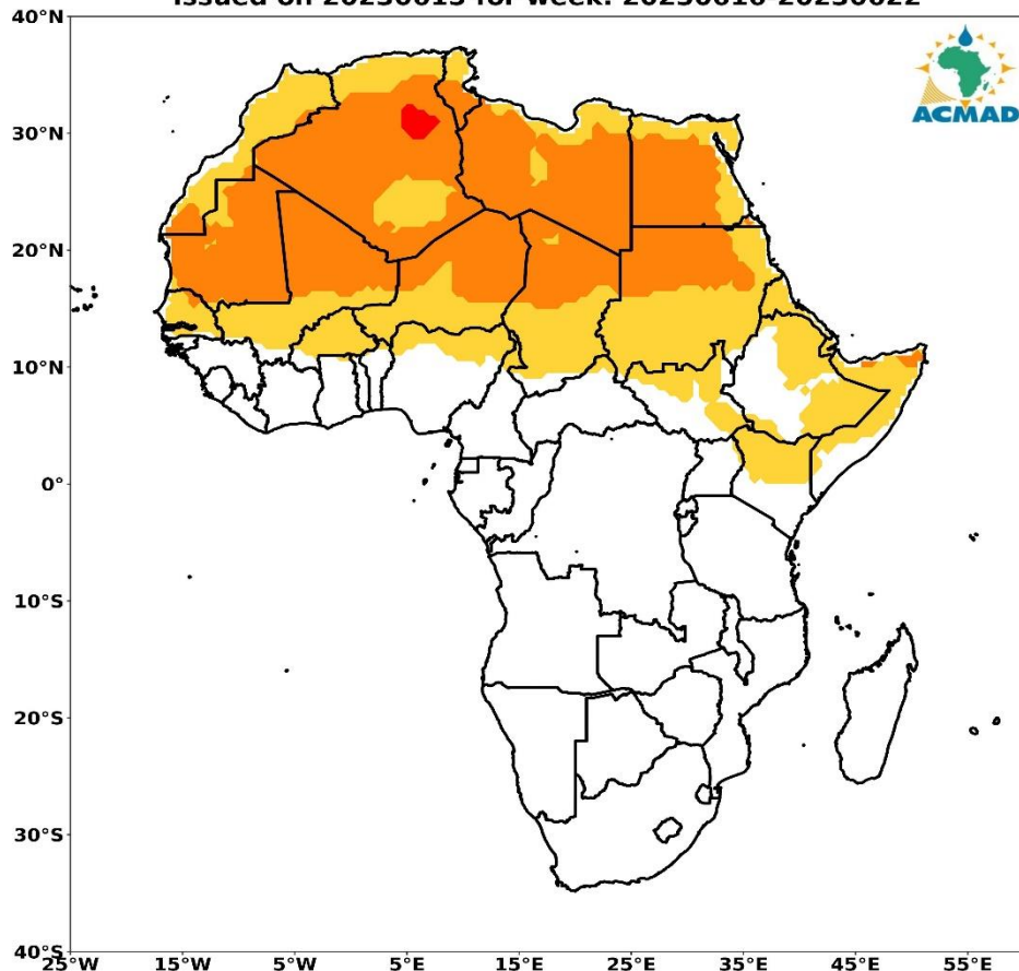
VIGILANCE MAP FOR MENINGITIS OUTBREAKS IN AFRICA issued on 20230615 for week: 20230616-20230622
