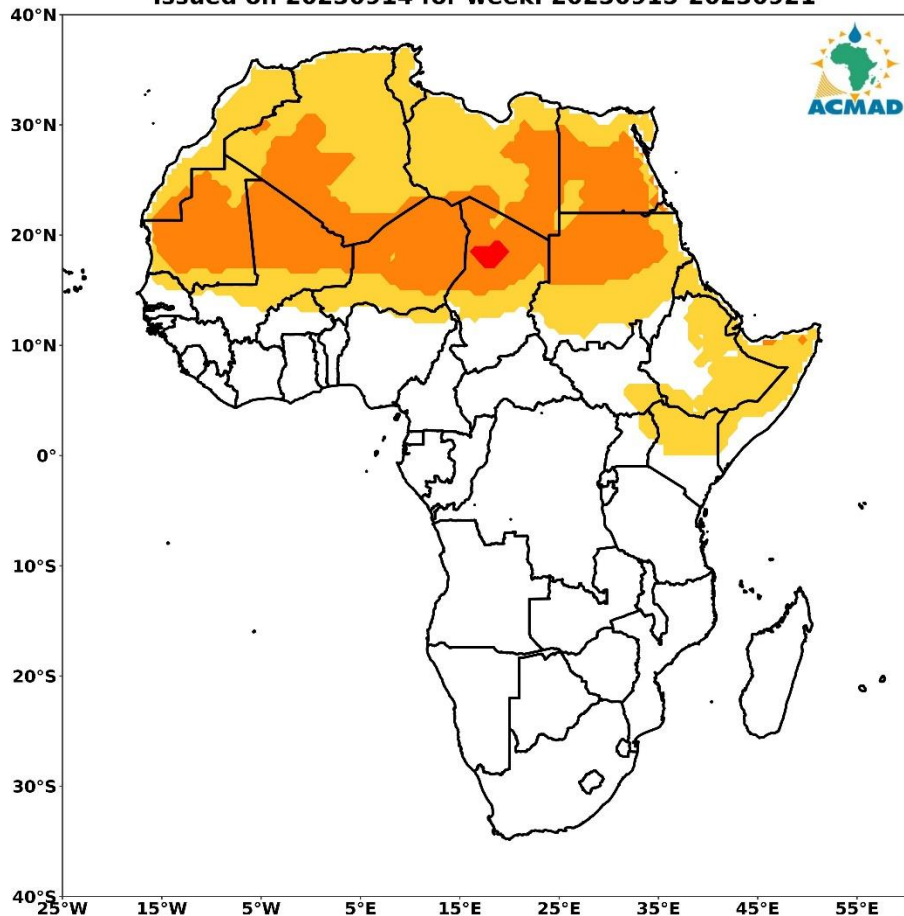
VIGILANCE MAP FOR MENINGITIS OUTBREAKS IN AFRICA issued on 20230914 for week: 20230915-20230921
