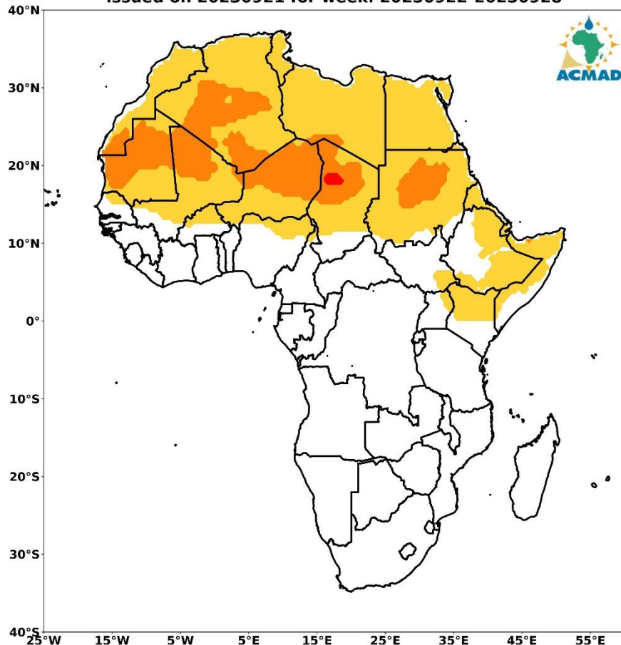
VIGILANCE MAP FOR MENINGITIS OUTBREAKS IN AFRICA issued on 20230921 for week: 20230922-20230928
