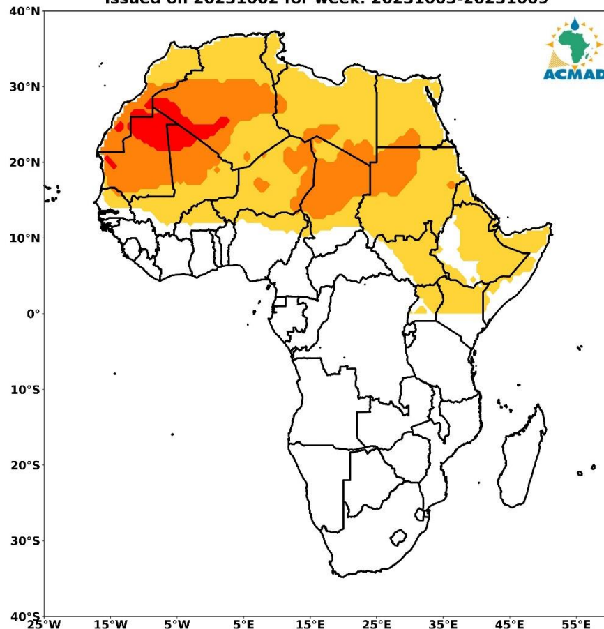
VIGILANCE MAP FOR MENINGITIS OUTBREAKS IN AFRICA issued on 20231002 for week: 20231003-20231009
