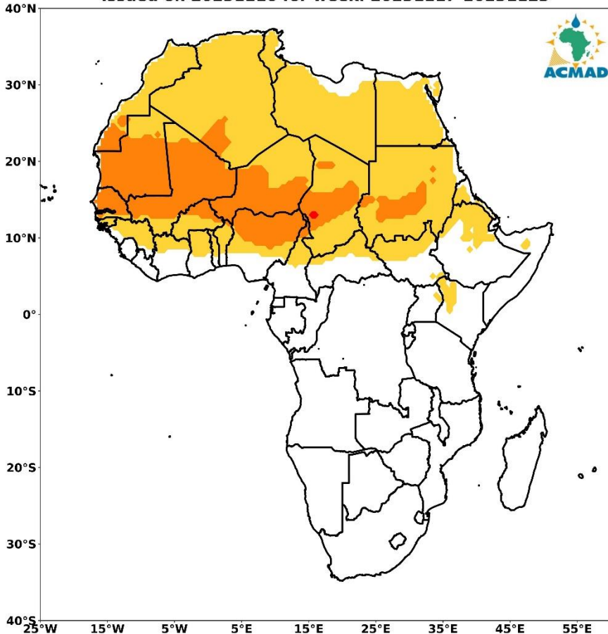
VIGILANCE MAP FOR MENINGITIS OUTBREAKS IN AFRICA issued on 20231116 for week: 20231117-20231123
