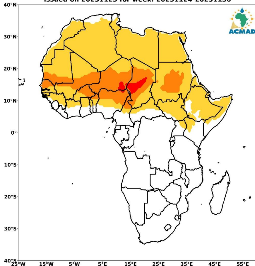
VIGILANCE MAP FOR MENINGITIS OUTBREAKS IN AFRICA issued on 20231123 for week: 20231124-20231130
