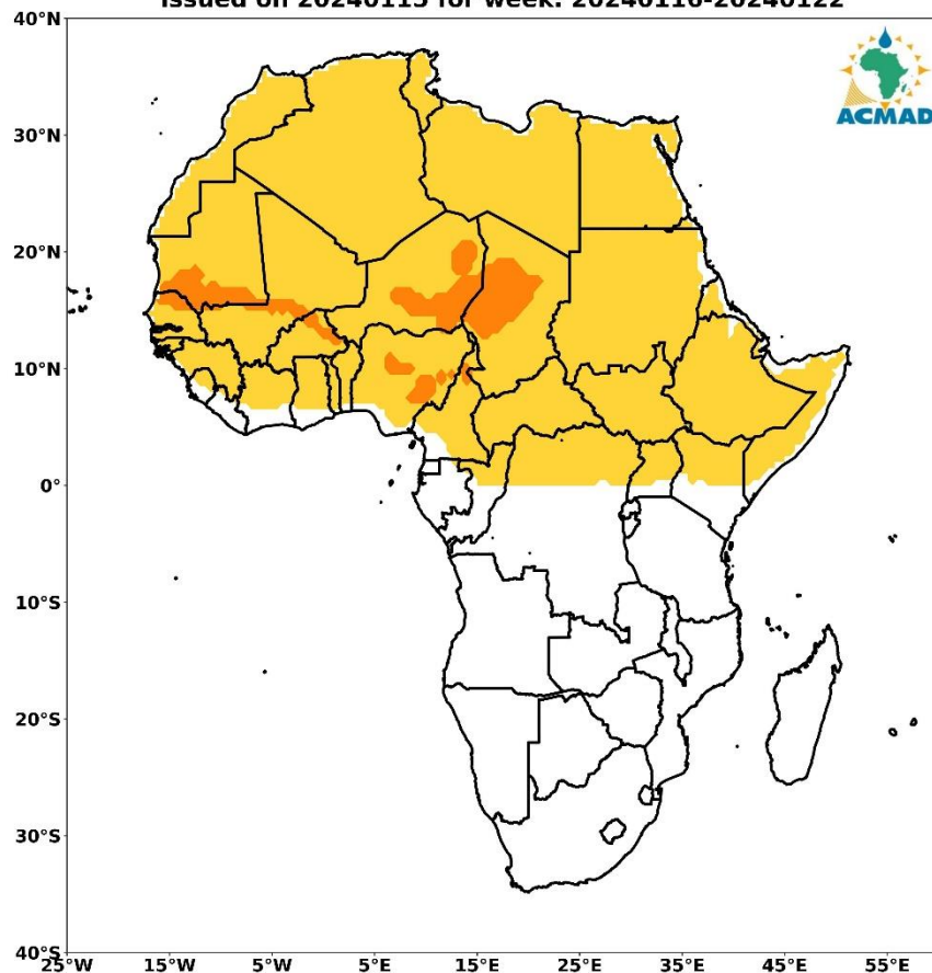
VIGILANCE MAP FOR MENINGITIS OUTBREAKS IN AFRICA issued on 20240115 for week: 20240116-20240122
