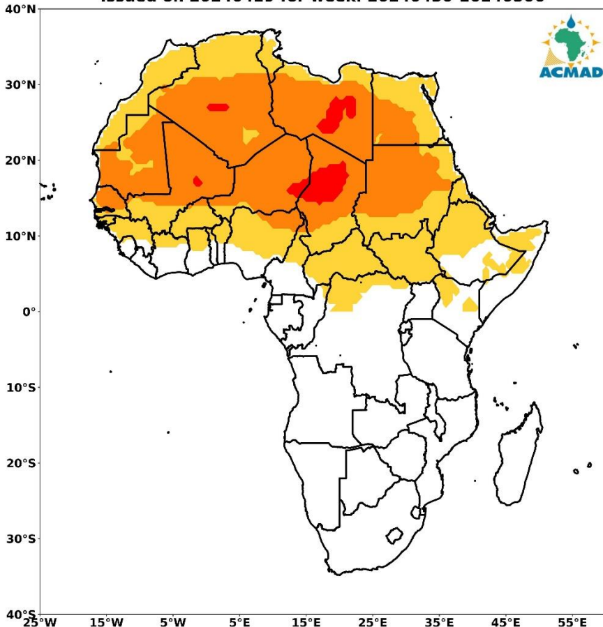
VIGILANCE MAP FOR MENINGITIS OUTBREAKS IN AFRICA issued on 20240429 for week: 20240430-20240506
