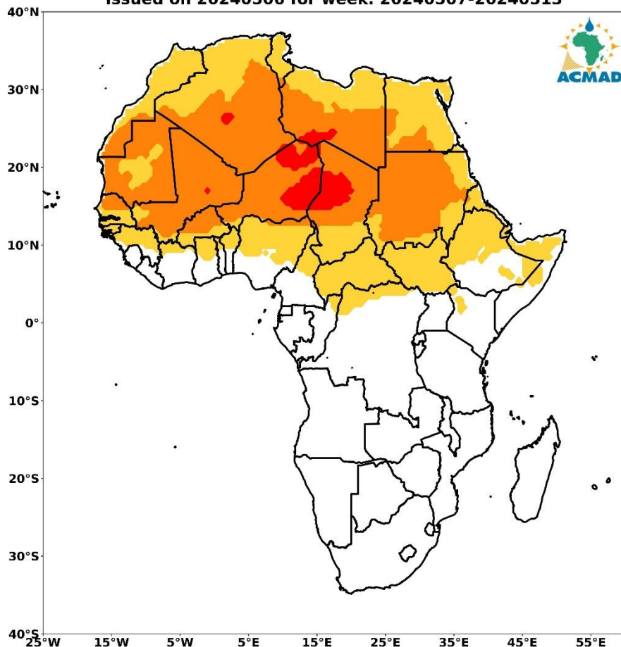
VIGILANCE MAP FOR MENINGITIS OUTBREAKS IN AFRICA issued on 20240506 for week: 20240507-20240513
