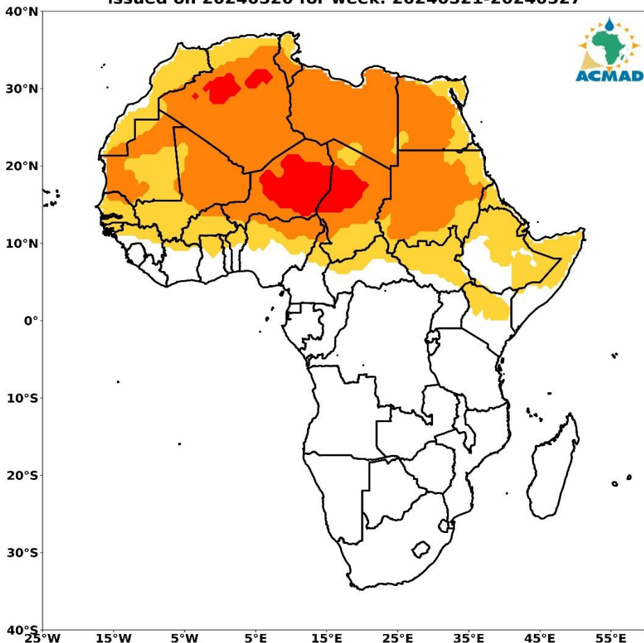
VIGILANCE MAP FOR MENINGITIS OUTBREAKS IN AFRICA issued on 20240520 for week: 20240521-20240527
