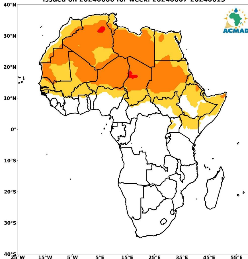
VIGILANCE MAP FOR MENINGITIS OUTBREAKS IN AFRICA issued on 20240606 for week: 20240607-20240613
