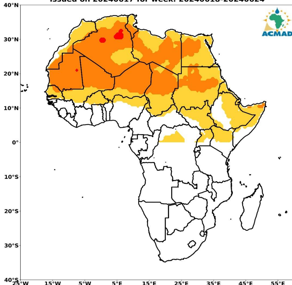
VIGILANCE MAP FOR MENINGITIS OUTBREAKS IN AFRICA issued on 20240617 for week: 20240618-20240624
