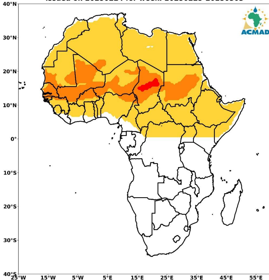
VIGILANCE MAP FOR MENINGITIS OUTBREAKS IN AFRICA issued on 20250224 for week: 20250225-20250303
