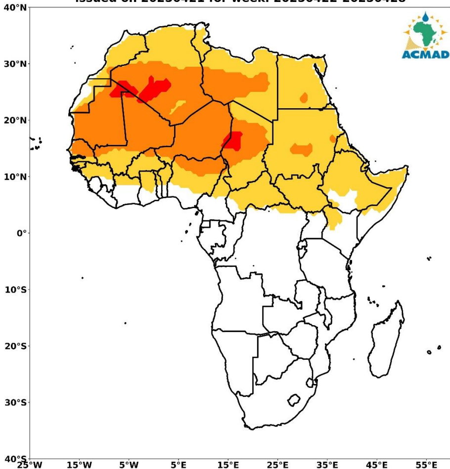
VIGILANCE MAP FOR MENINGITIS OUTBREAKS IN AFRICA issued on 20250421 for week: 20250422-20250428
