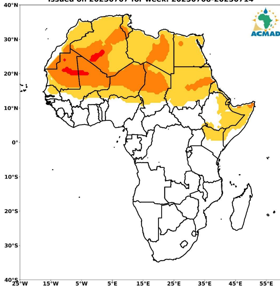
VIGILANCE MAP FOR MENINGITIS OUTBREAKS IN AFRICA issued on 20250707 for week: 20250708-20250714
