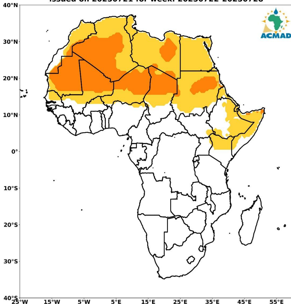
VIGILANCE MAP FOR MENINGITIS OUTBREAKS IN AFRICA issued on 20250721 for week: 20250722-20250728
